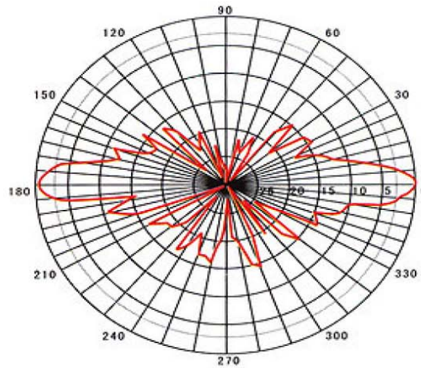
Horizontal pattern
